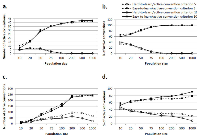
Figure 1. Absolute number (left panels) and relative proportion (right panels) of active conventions after 1000 iterations, obtained for increasing values of population sizes (displayed in the x -axis). Top panels (a. and b.) display the results corresponding to a value M_{max}=100 (the maximum number of convention-tokens that an agent can store in memory), while bottom panels (c. and d.), display the results corresponding to a value M_{max}=500 . Filled squares correspond to Easy-to-learn conventions, and open circles correspond to Hard-to-learn conventions. Results displayed in dashed lines correspond to active-convention criterion = 5 agents, and solid lines to active-convention criterion = 10 agents.
